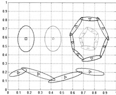
Fig.6 Learning output of LD-SOINN [33]
