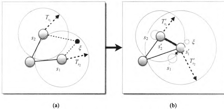
Fig.4 Updating the weights of neurons
