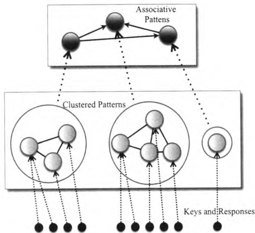
Fig.8 Network structure of GAM
