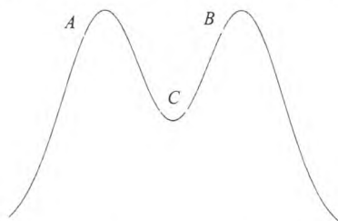
Fig.5 Overlapped density
