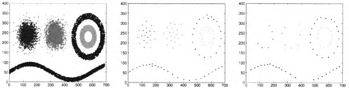
Fig.7 ASC trained by artificial data [31]
